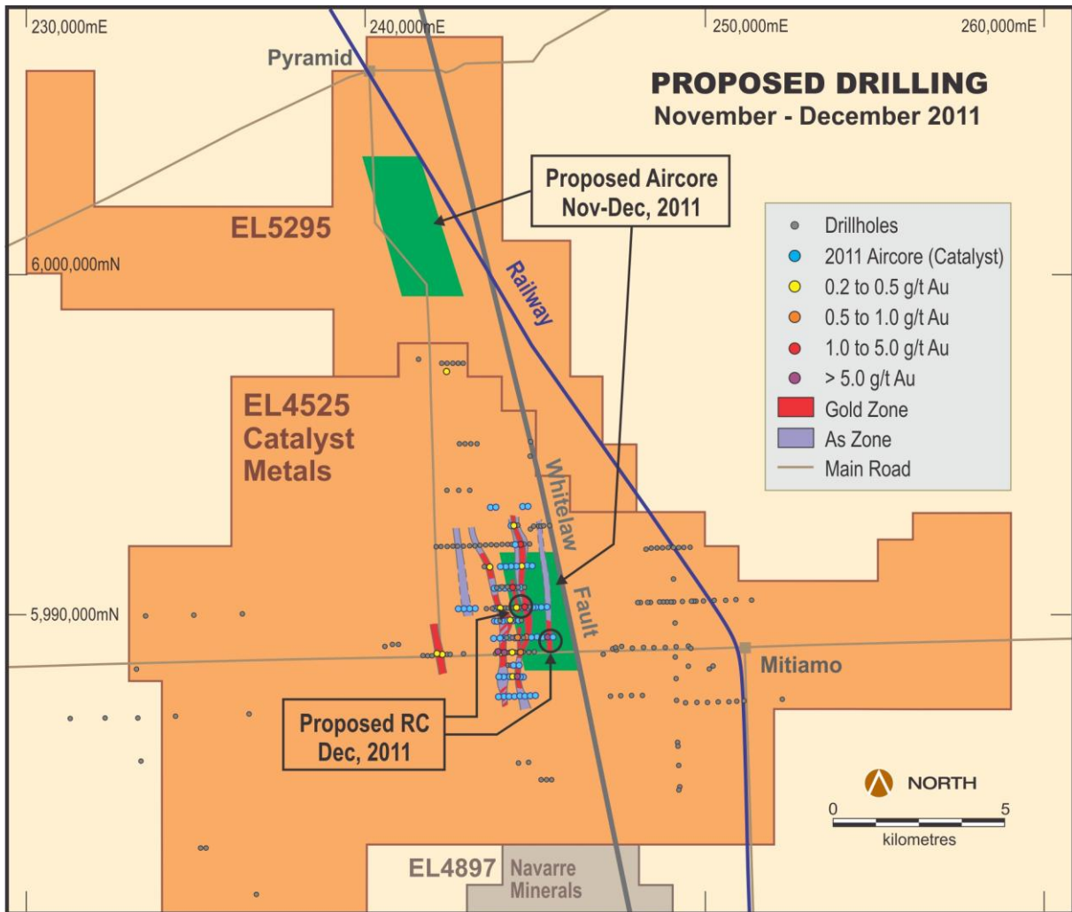
Figure 1 – Proposed Aircore & RC Drilling for November & December 2011
